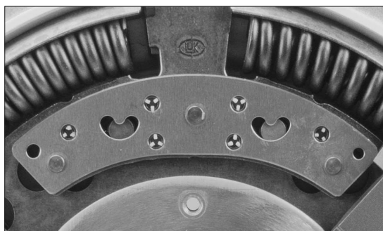
Image 2: Centrifugal-force pendulum
